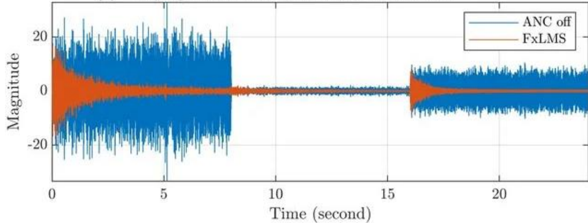
Varying noise cancellation based on FxLMS
