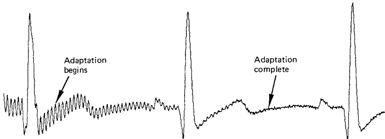
Output of Neural Network Filter
